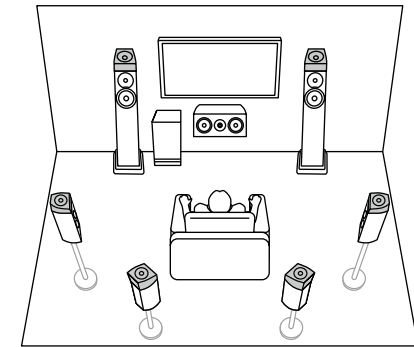
7.1.2 ch (Dolby Enabled Speakers (Front or Surround or Surround Back)) (→p36)
