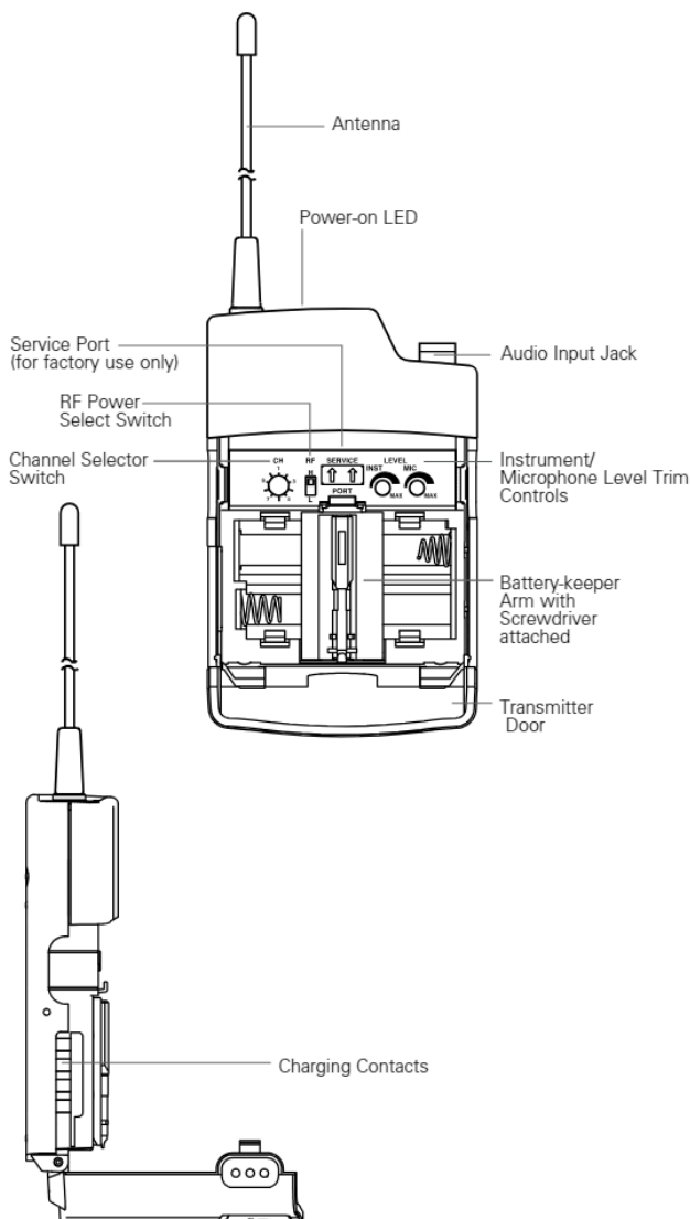
Fig. E – UniPak® Transmitter Open
