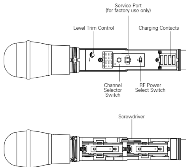
Fig. 1 – Handheld Transmitter Interior View
