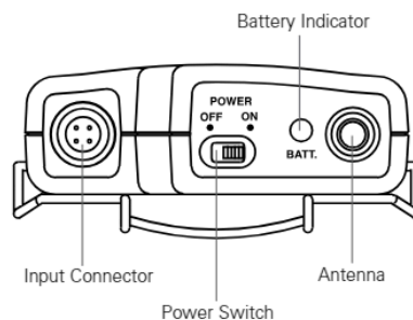
Fig. G – UniPak Transmitter Top View
