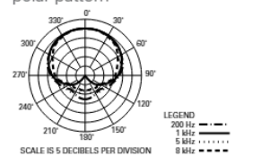
polar pattern
