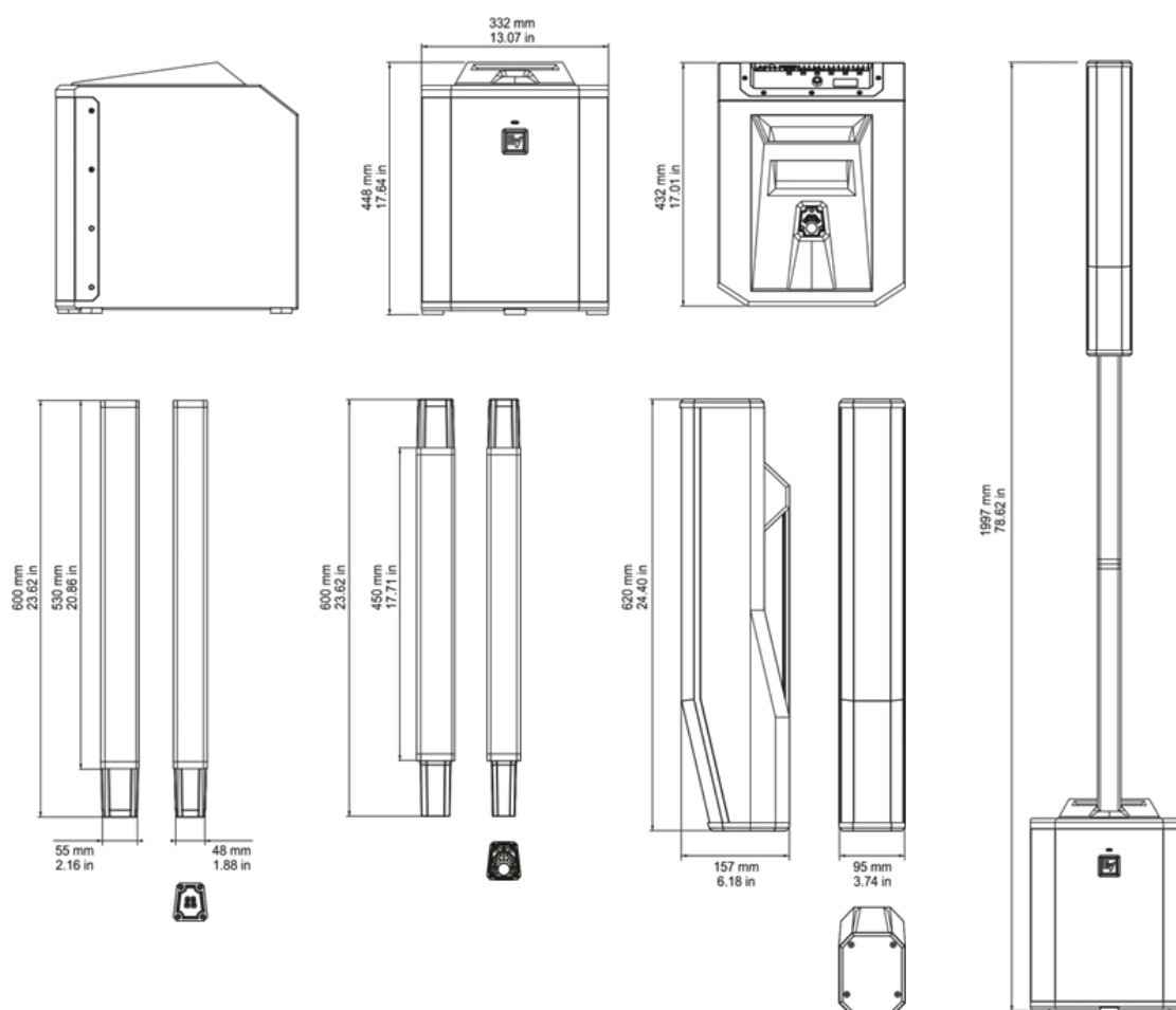
Figure 10.2: Dimensions EVOLVE 30M
