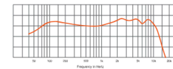
LEGEND: 12" or more on axis
